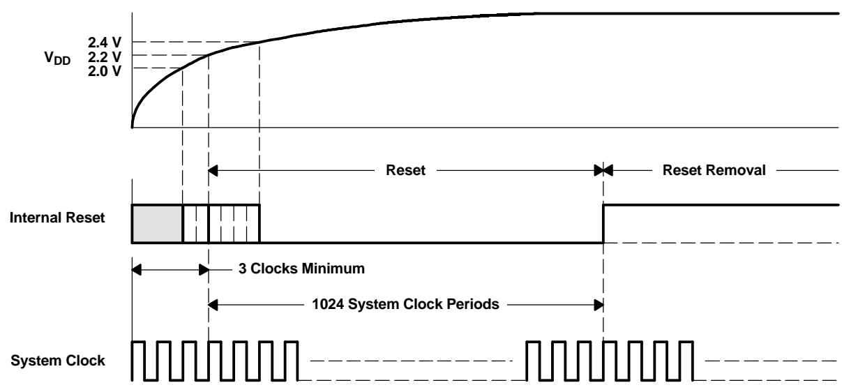
Figure 45. Internal Power-On Reset Timing
