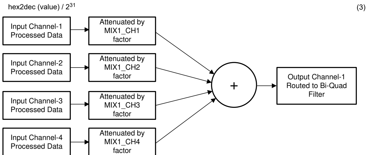
Figure 8-24. Programmable Digital Mixer Block Diagram
