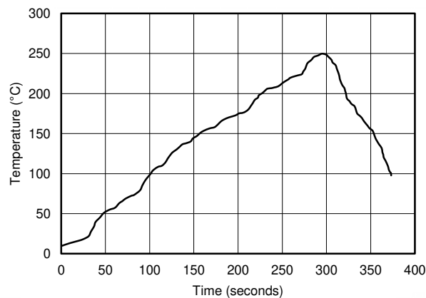
Figure 7-12. Reflow Profile
