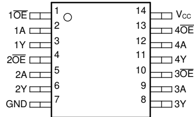
Figure 4-1. PW Package, 14-Pin TSSOP (Top View)
