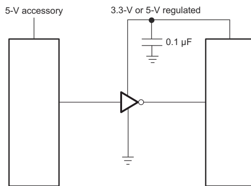
Figure 8-1. Typical Application Schematic
