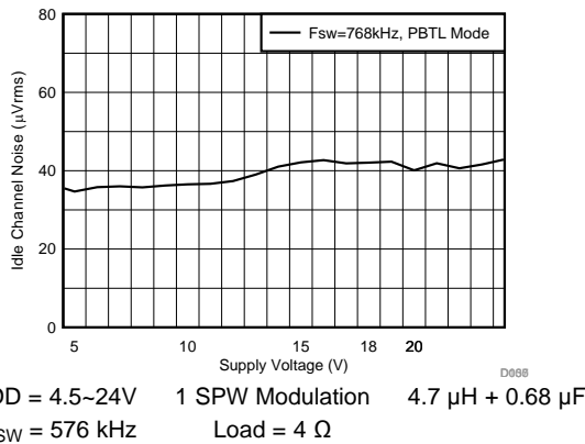
Figure 51. Idle Channel Noise vs Supply Voltage
