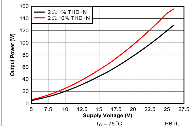
Figure 7-32. Output Power vs Supply Voltage - PBTL
