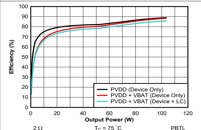
Figure 7-33. Efficiency vs Output Power - PBTL - 2 Ohm
