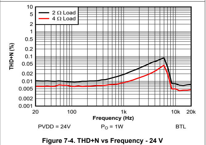
Figure 7-4. THD+N vs Frequency - 24V
