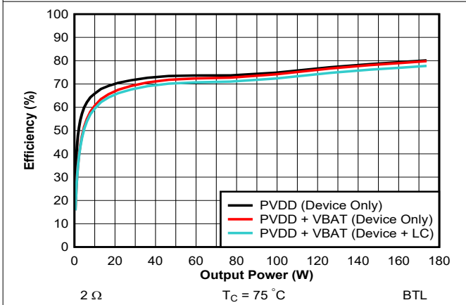
Figure 7-9. Efficiency vs Output Power - 14.4 V - 2 \Omega
