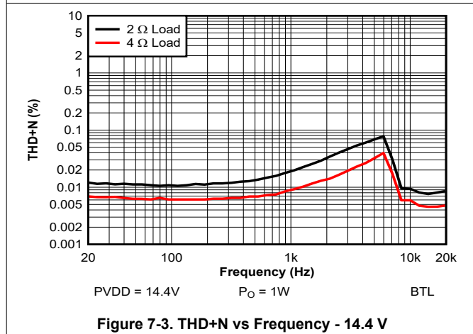
Figure 7-3. THD+N vs Frequency - 14.4V
