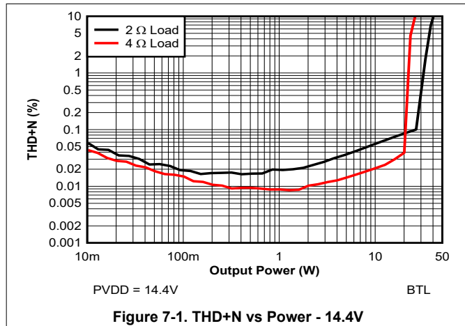
Figure 7-1. THD+N vs Power - 14.4V
