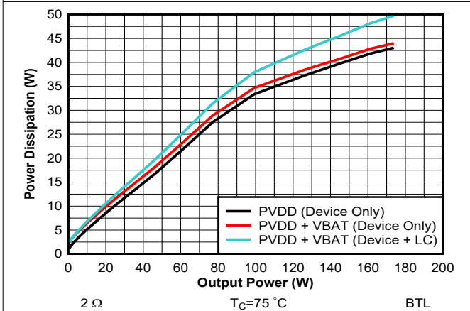
Figure 7-11. Power Dissipation vs Output Power - 14.4 V - 2 \Omega
