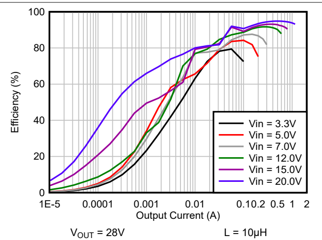
Figure 6-2. Efficiency vs Output Current, V_{OUT} = 28\text{V}
