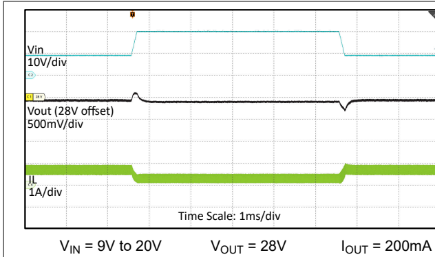
Figure 8-17. Line Transient
