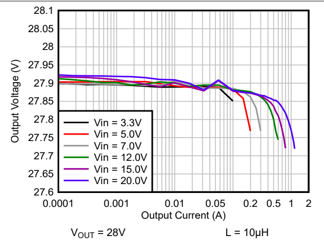
Figure 6-4. Load regulation, V_{OUT} = 28\text{V}
