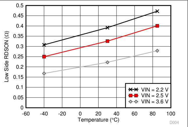
Figure 7-4. Low-side R_{DS(on)} vs Temperature
