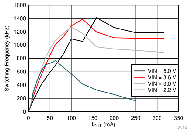
Figure 9-6. Switching Frequency vs Load Current V_{OUT} = 1.8\text{ V}
