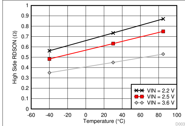
Figure 7-3. High Side R_{DS(on)} vs Temperature
