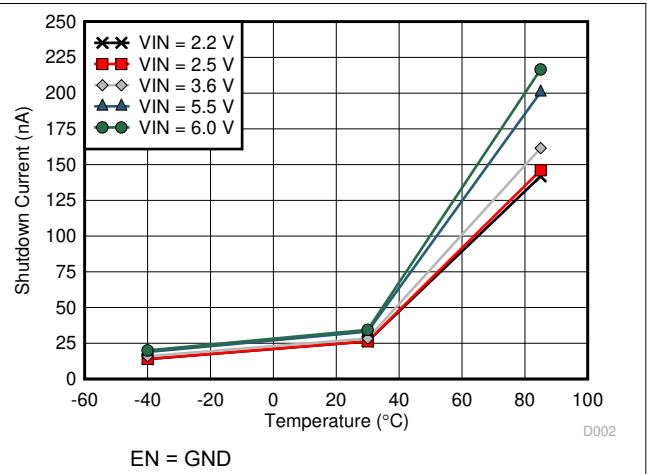
Figure 7-2. Shutdown Current I_{SD} vs Temperature
