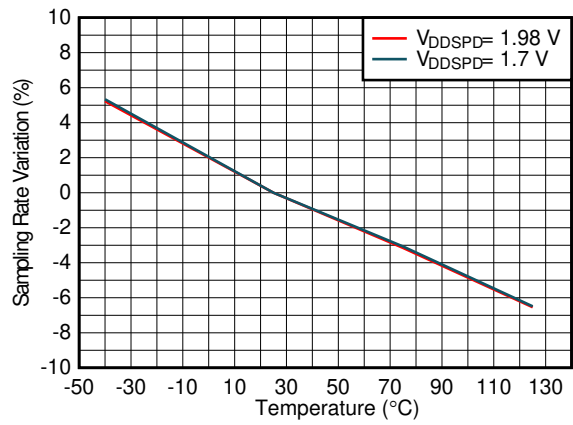
Figure 6-13. Sampling Rate Change
