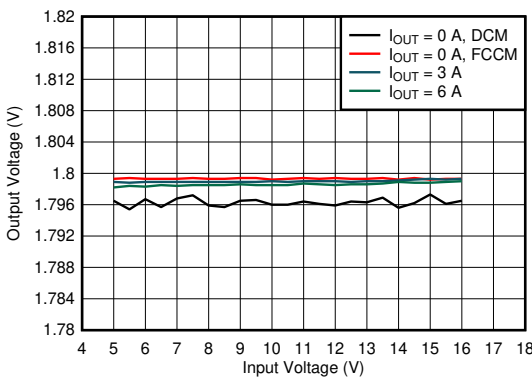
V_{OUT} = 1.8\text{ V} f_{SW} = 1100\text{ kHz}
