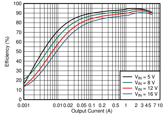
V_{OUT} = 1.8\text{ V} f_{SW} = 600\text{ kHz} MODE = DCM VCC = Int 3.0 V
