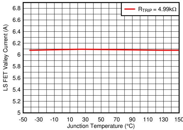
Figure 5-3. Overcurrent Limit
