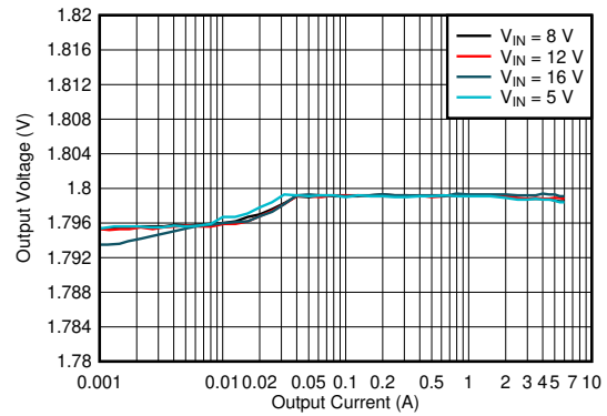
V_{OUT} = 1.8\text{ V} f_{SW} = 1100\text{ kHz} MODE = DCM
