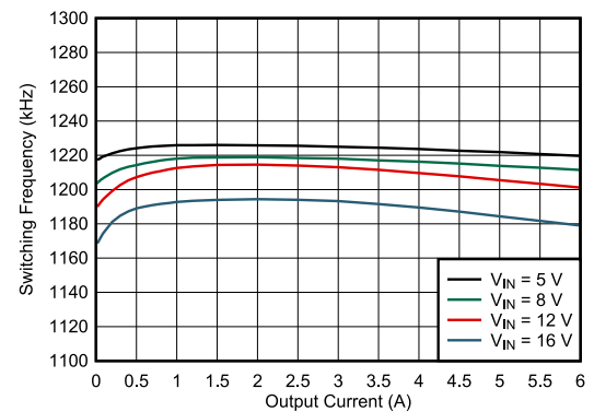
V_{OUT} = 1.8\text{ V} f_{SW} = 1100\text{ kHz} MODE = FCCM
