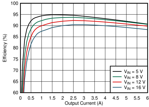
V_{OUT} = 1.8\text{ V} f_{SW} = 600\text{ kHz} MODE = FCCM VCC = Int 3.0 V
