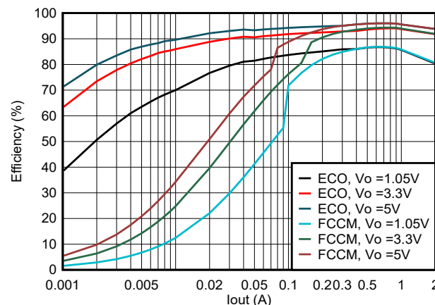
TPS56224x Efficiency at Vin = 12V
