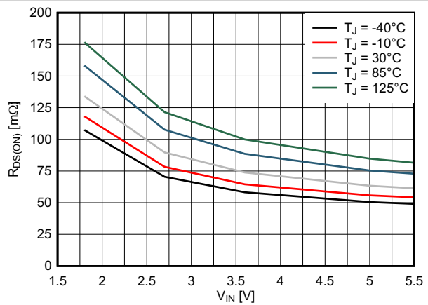
Figure 6-6. Low-Side Switch Drain Source Resistance, R_{DS(ON)}
