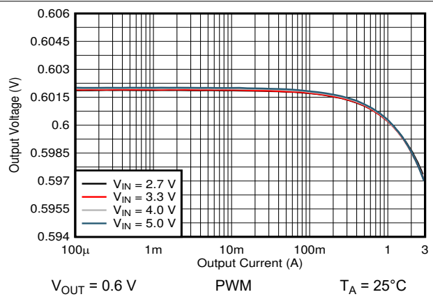
Figure 9-17. Output Voltage Versus Output Current
