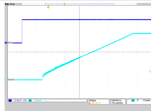
Figure 9-53. Start-Up Timing
