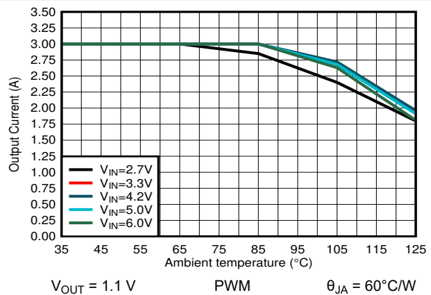
Figure 9-19. Output Current Versus Ambient Temperature
