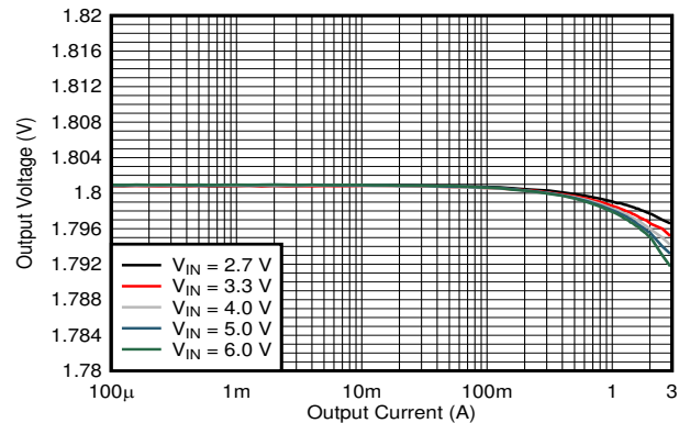
Figure 9-11. Output Voltage Versus Output Current
