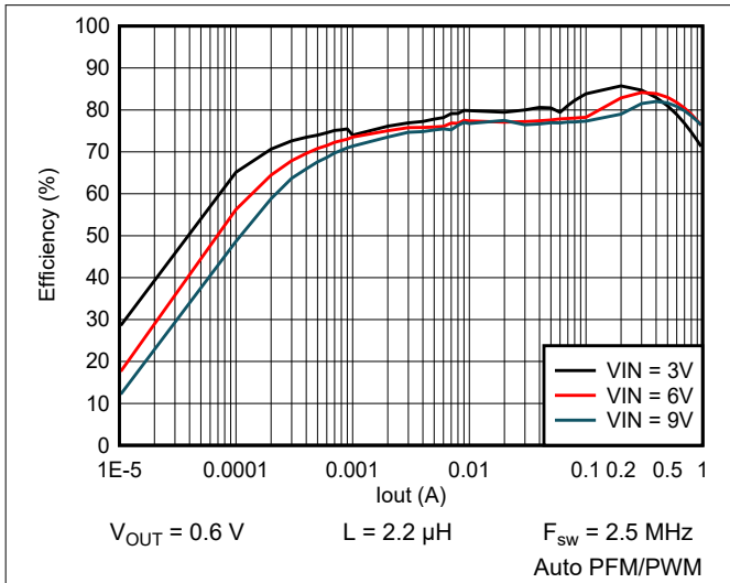
Figure 9-50. Efficiency vs Output Current
