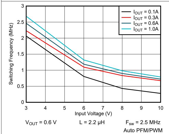
Figure 9-52. Switching Frequency vs Input Voltage
