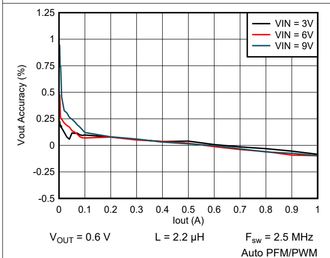
Figure 9-54. Output Voltage vs Output Current
