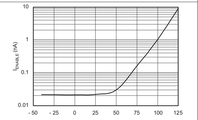
Figure 24. I_{ENABLE} vs Temperature
