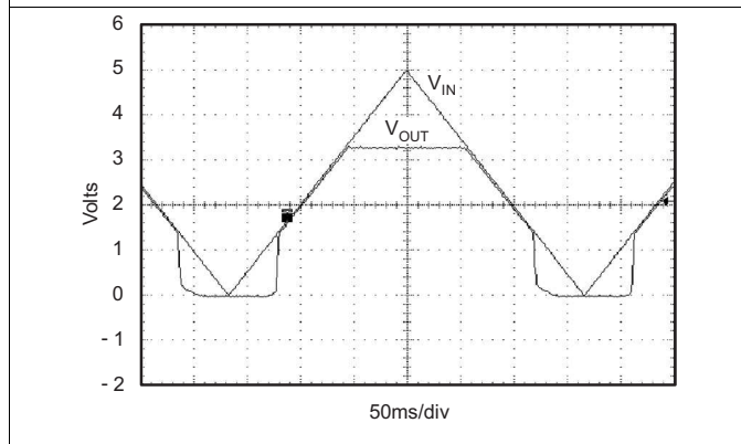
Figure 23. TPS73233-Q1 – Power Up and Power Down
