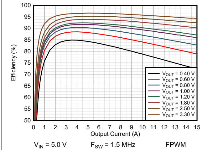
Figure 9-18. Efficiency TPSM8287A15BAH
