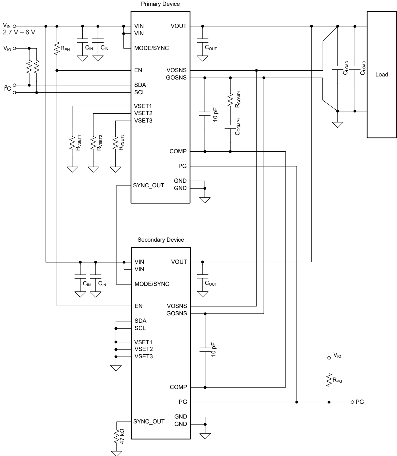
Figure 7-22. Two TPSM8287Axx Devices in a Stacked Configuration
