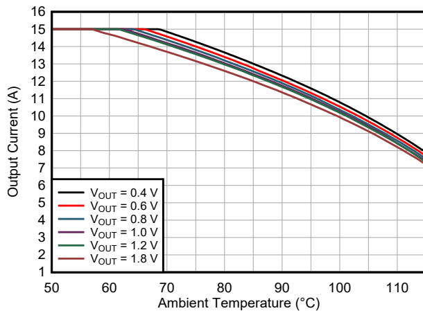
Figure 9-46. Safe Operating Area TPSM8287A15BAH V_{IN} = 3.3\text{ V}
