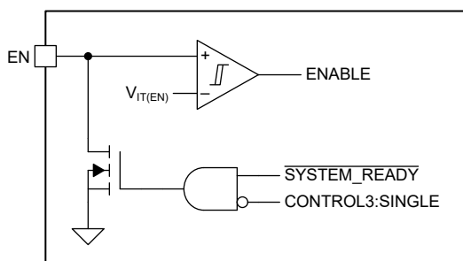
Figure 7-10. Enable Functional Block Diagram
