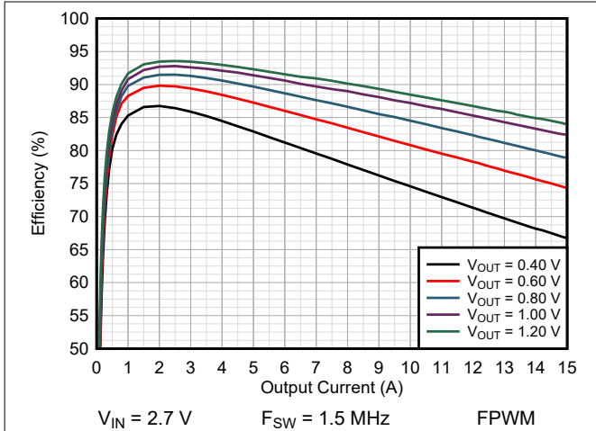
Figure 9-14. Efficiency TPSM8287A15BAH
