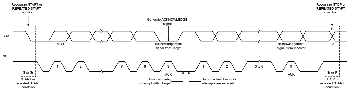
Figure 7-26. Bus Protocol
