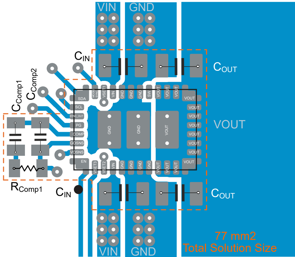
Figure 9-57. Layout Example
