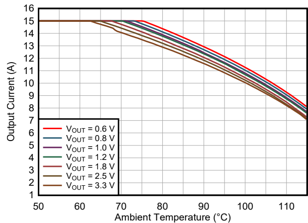
Figure 9-47. Safe Operating Area TPSM8287A15BAH V_{IN} = 5.0\text{ V}
