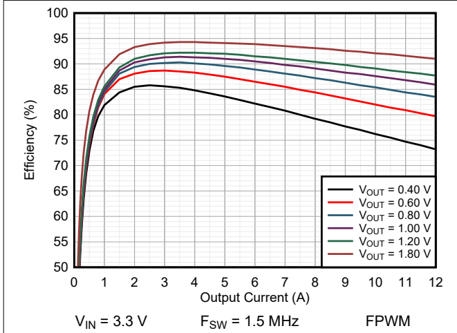
Figure 9-10. Efficiency TPSM8287A12BAS
