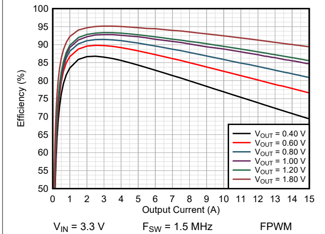
Figure 9-16. Efficiency TPSM8287A15BAH
