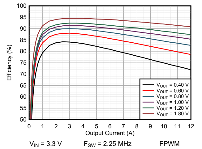
Figure 9-11. Efficiency TPSM8287A12BBS
