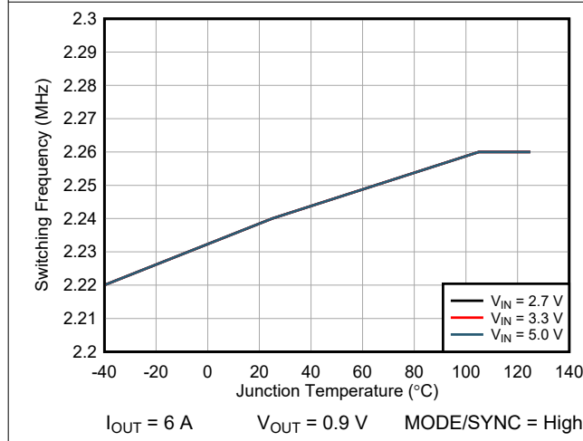
Figure 6-3. TPSM8287A12BBS Switching Frequency vs T_J
