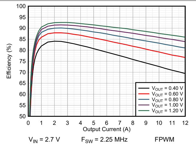
Figure 9-9. Efficiency TPSM8287A12BBS
