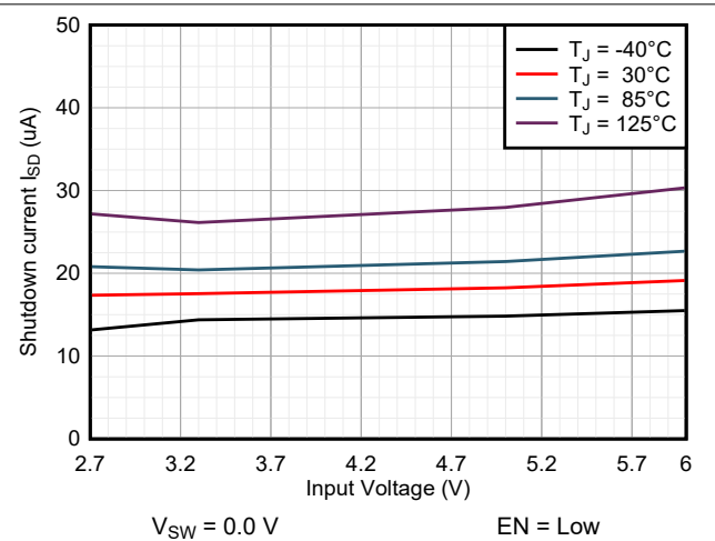
Figure 6-2. Shutdown Current
