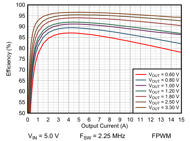
Figure 9-19. Efficiency TPSM8287A15BBH
