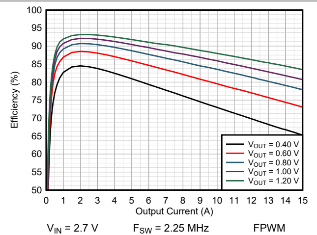
Figure 9-15. Efficiency TPSM8287A15BBH
