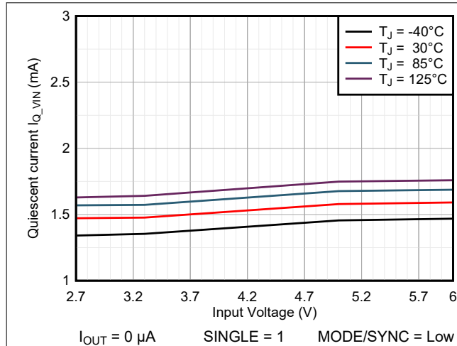
Figure 6-1. Operating Supply Current (Power-Save Mode)
