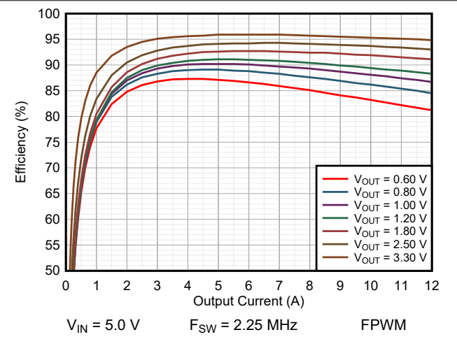
Figure 9-13. Efficiency TPSM8287A12BBS
