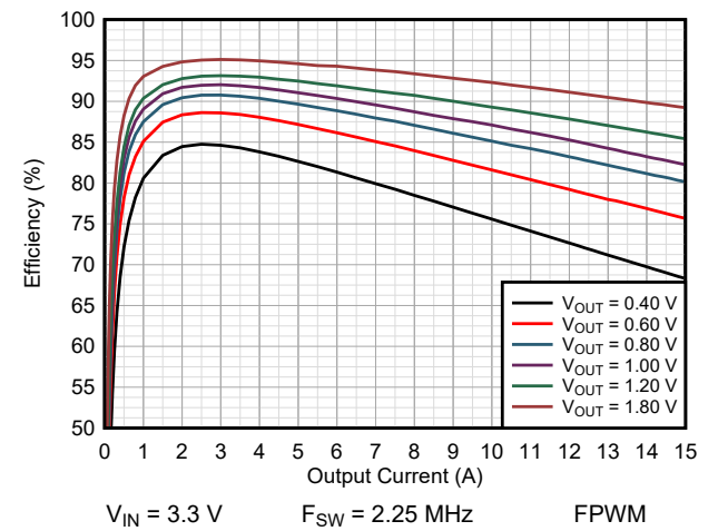
Figure 9-17. Efficiency TPSM8287A15BBH
