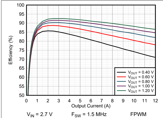
Figure 9-8. Efficiency TPSM8287A12BAS
