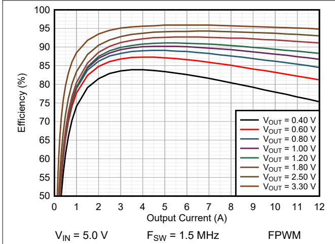
Figure 9-12. Efficiency TPSM8287A12BAS
