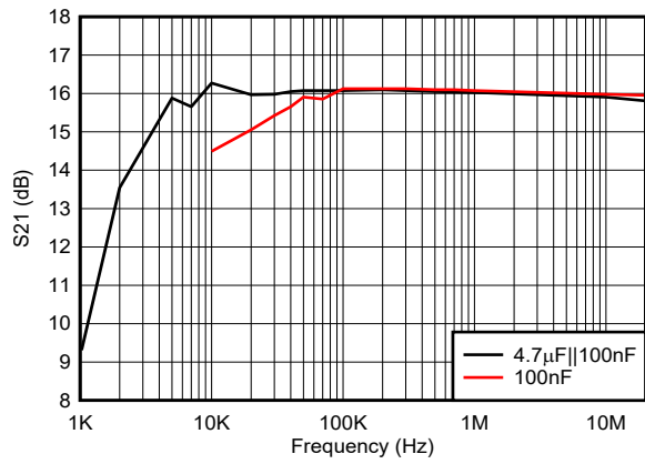
Low frequency cut-off as a function of ac-coupling cap Figure 5-37. Low Frequency Gain Response
