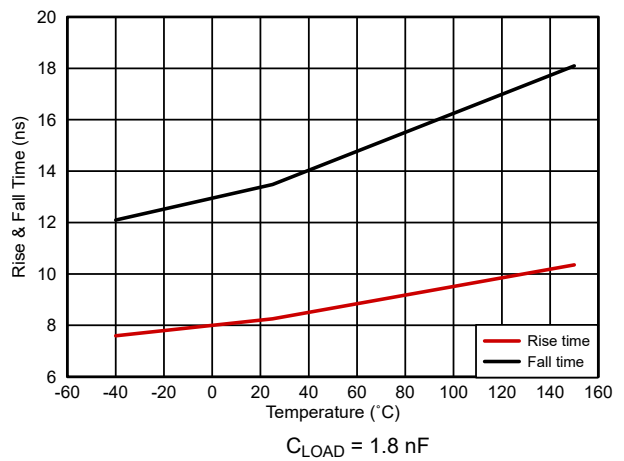
Figure 5-16. Output Rise and Fall Time
