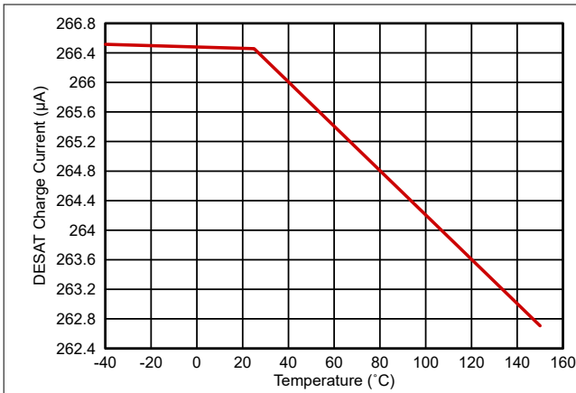
Figure 5-23. DESAT Charge Current vs Temperature
