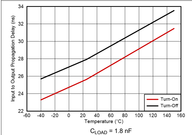
Figure 5-19. Input Propagation Delay
