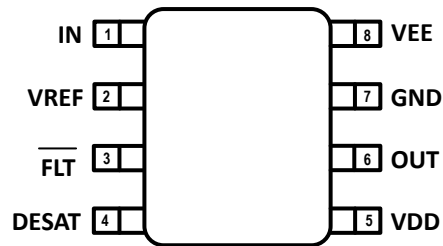
Figure 4-1. UCC57102Z-Q1 D Package SOIC-8 Top View
