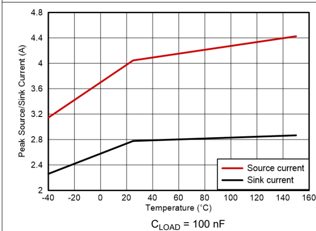
Figure 5-25. Peak Source and Sink Current
