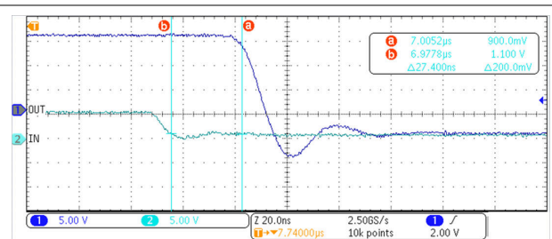
Figure 7-4. UCC57102Z-Q1 Falling (Turn-Off) Propagation Delay
