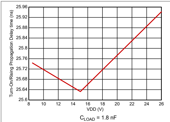
Figure 5-17. Input to Output Rising (Turnon) Propagation Delay
