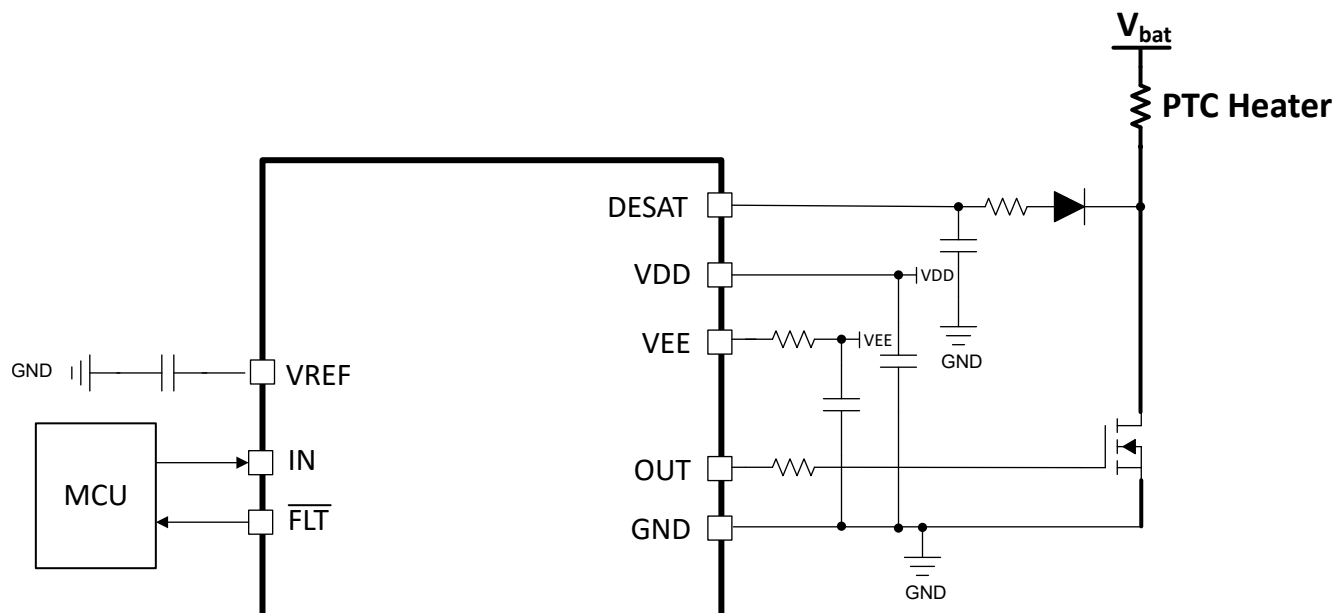
Figure 7-1. UCC57102Z-Q1 Used in a PTC Heater Application
