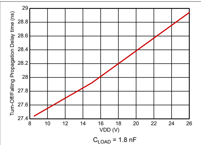
Figure 5-18. Input to Output Falling (Turnoff) Propagation Delay
