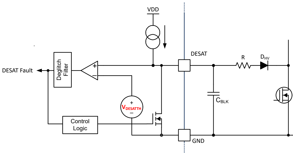
Figure 6-3. DESAT Protection
