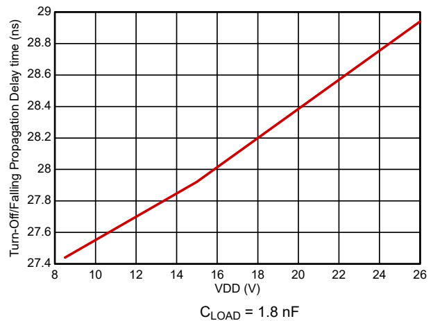
Figure 5-16. Input to Output Falling (Turnoff) Propagation Delay C LOAD = 1.8 nF
