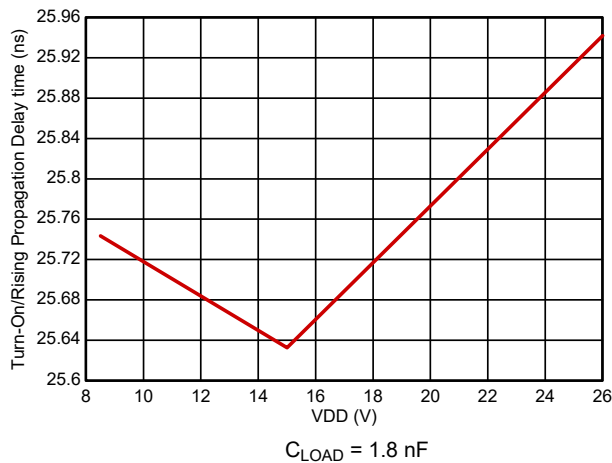
Figure 5-15. Input to Output Rising (Turnon) Propagation Delay C LOAD = 1.8 nF
