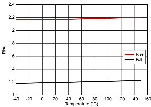
Figure 5-9. Input Threshold
