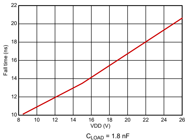
Figure 5-13. Output Fall Time C LOAD = 1.8 nF
