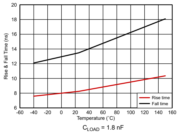
Figure 5-14. Output Rise and Fall Time C LOAD = 1.8 nF
