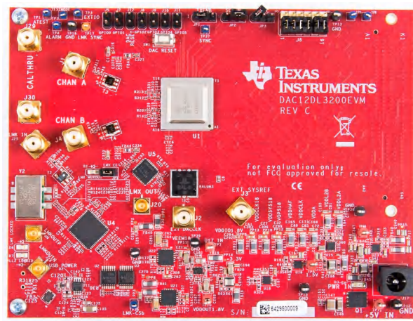
Figure 1-1. DAC12DL3200EVM
