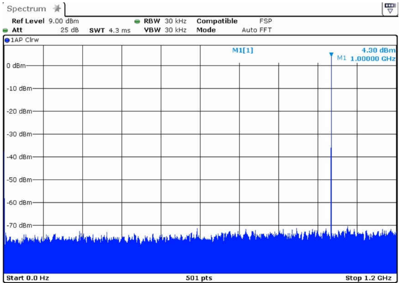
Figure 3-10. DAC Channel A Output
