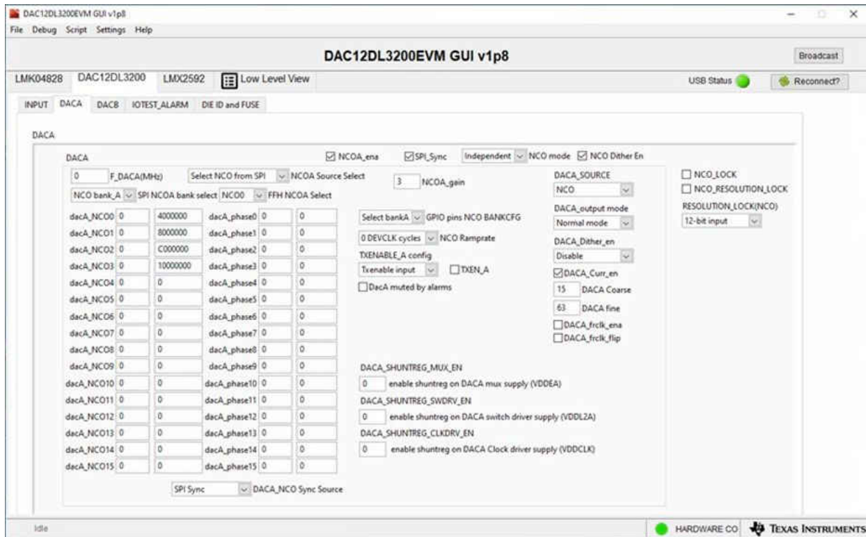
Figure 4-2. DAC Tab With NCO settings
