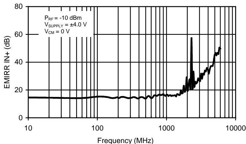
Figure 1. TLV2241 EMIRR IN+ vs Frequency
