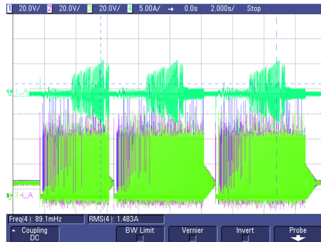
Figure 7. Auto BEMF Threshold Calculation
