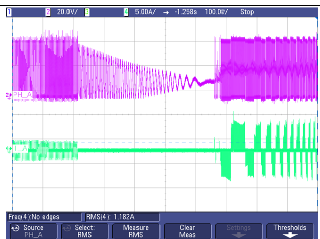
Figure 2. ISC Braking and Restarting Motor when Spinning in Reverse Direction
