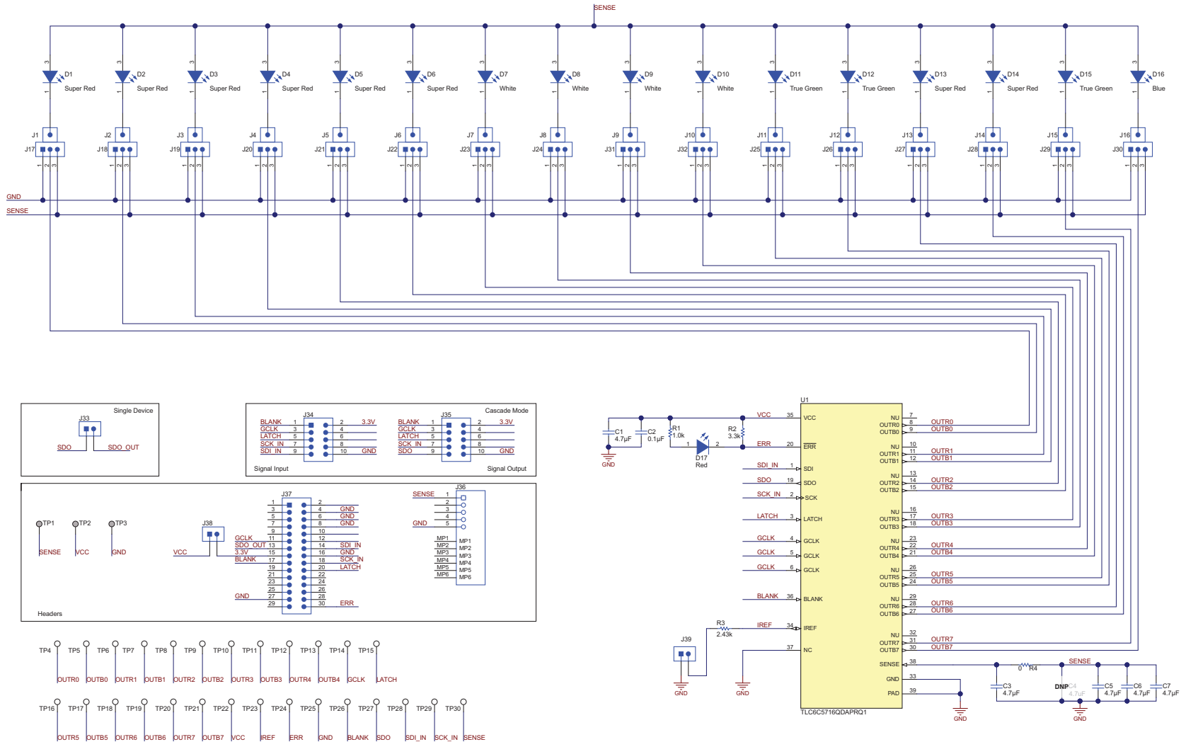
Figure 7. TLC6C5716EVM Schematic
