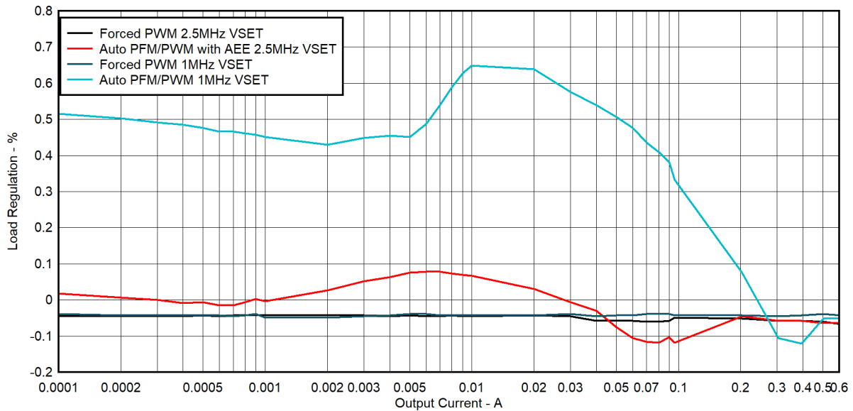
Figure 5-2. Load Regulation, V_{IN} = 12\text{ V} , V_{OUT} = 3.3\text{ V} , F_{SW} = 2.5\text{ MHz} and 1\text{ MHz}
