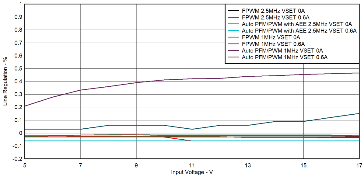
Figure 5-3. Line Regulation, V_{IN} = 5\text{ V}–17\text{ V} , V_{OUT} = 3.3\text{ V} , I_{OUT} = 0\text{ A} and 600\text{ mA} , F_{SW} = 2.5\text{ MHz} and 1\text{ MHz}
