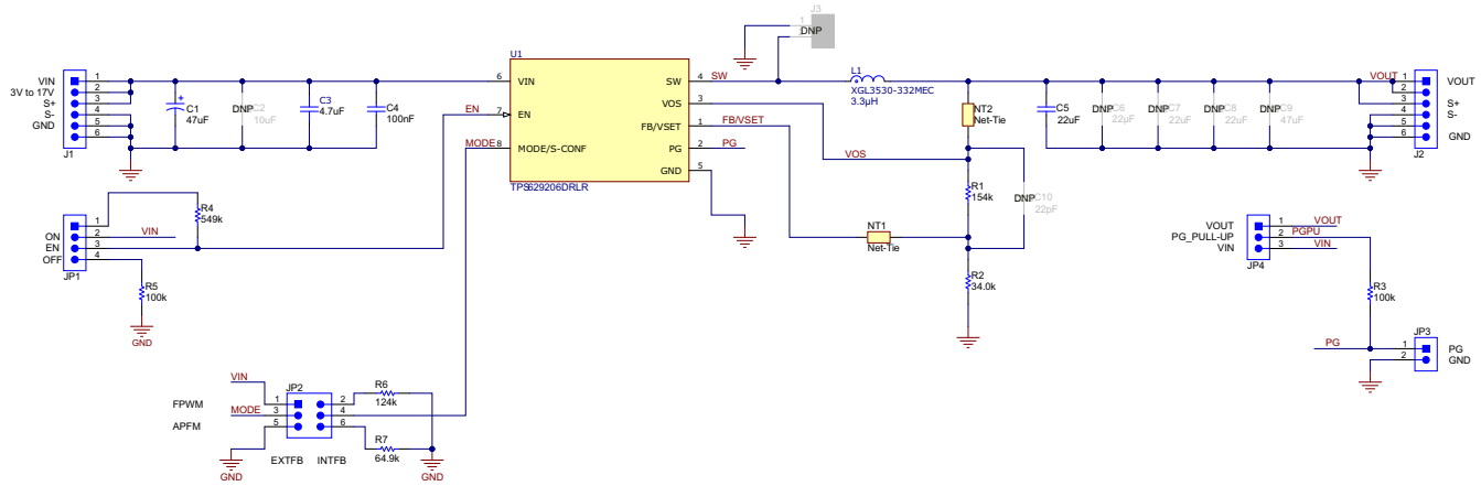
Figure 7-1. TPS629206EVM Schematic
