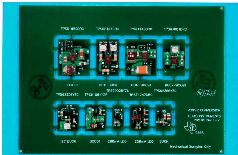
Power Conversion Nano-Evaluation Module – Top Side View
