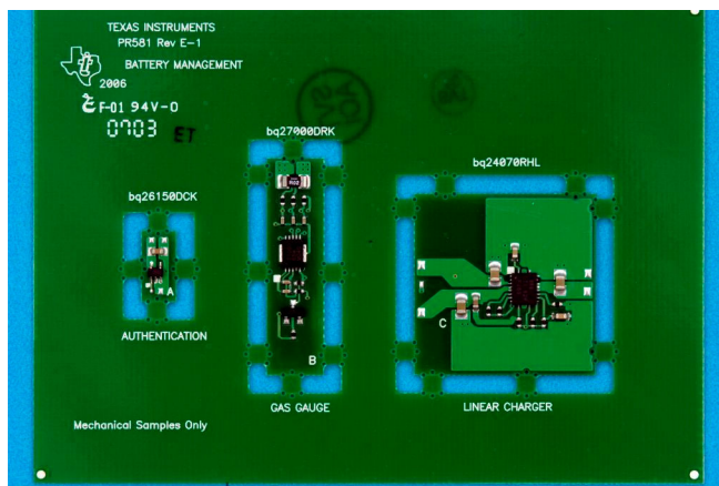
Battery Management Nano-Evaluation Module – Top Side View
