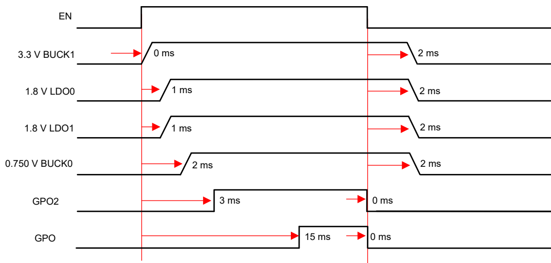
Figure 3-1. LP873364 Power-up and Power Down Sequence
