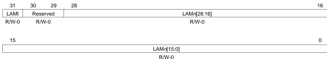
Figure 2-35. Local-Acceptance-Mask Register (LAM n )
