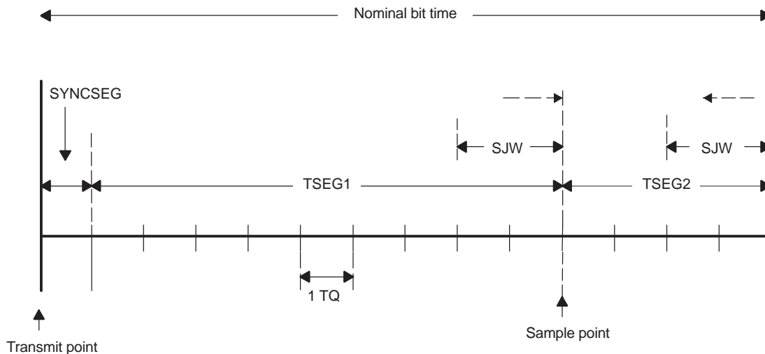
Figure 3-2. CAN Bit Timing
