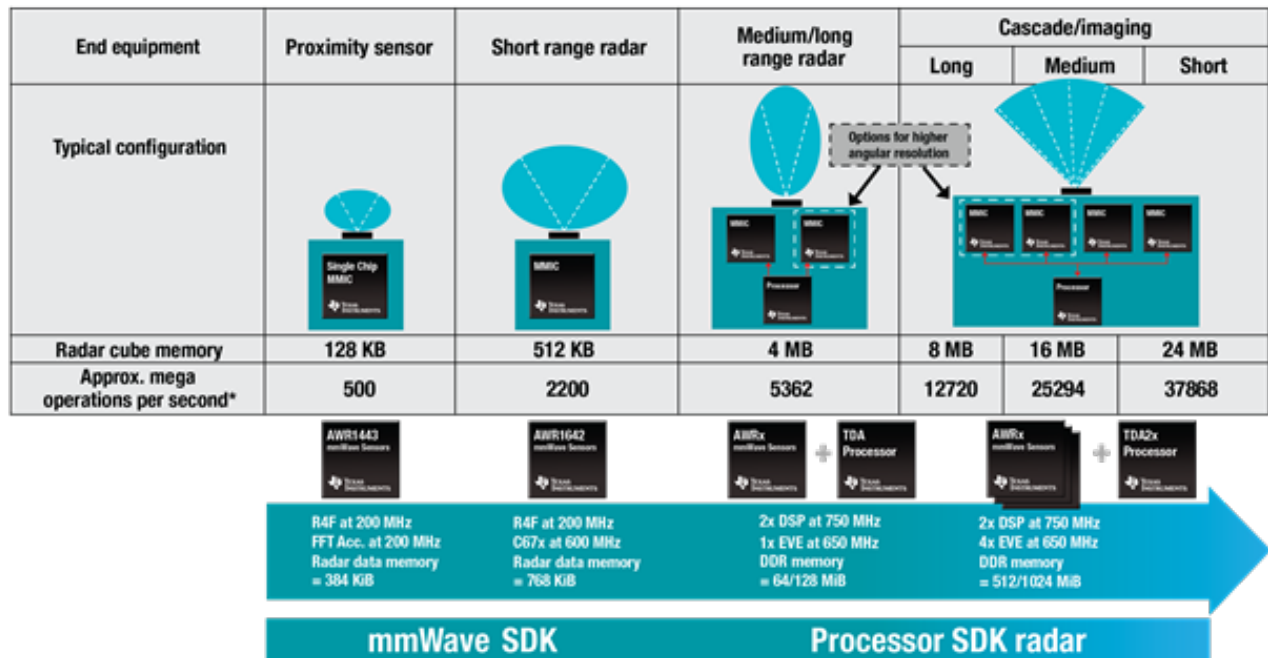
Figure 5. Radar Configuration with Memory and Processing Trends
