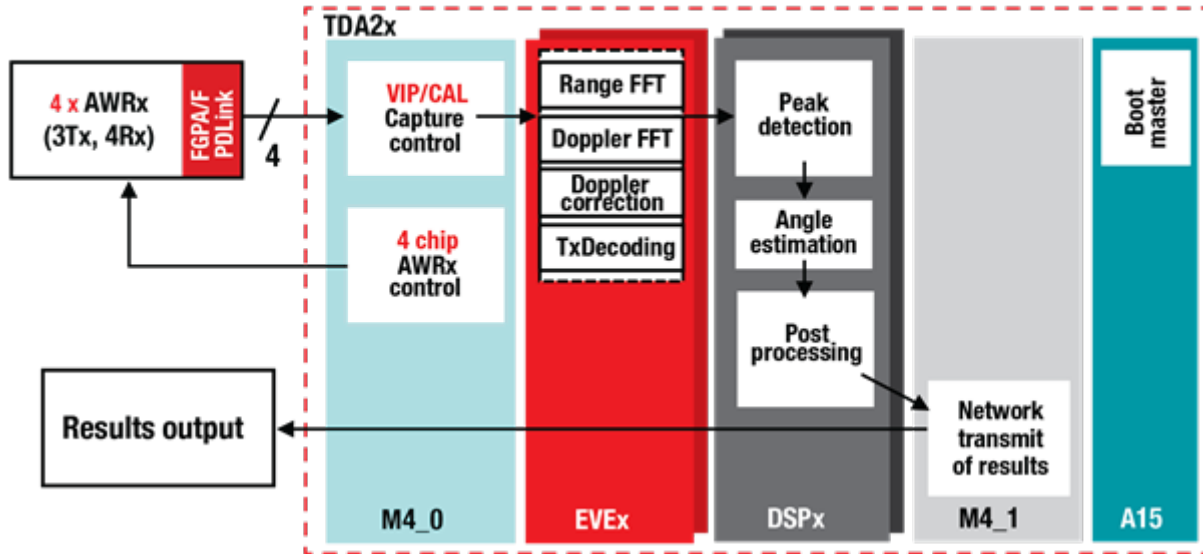
Figure 4. Radar Data Processing Flow Partition
