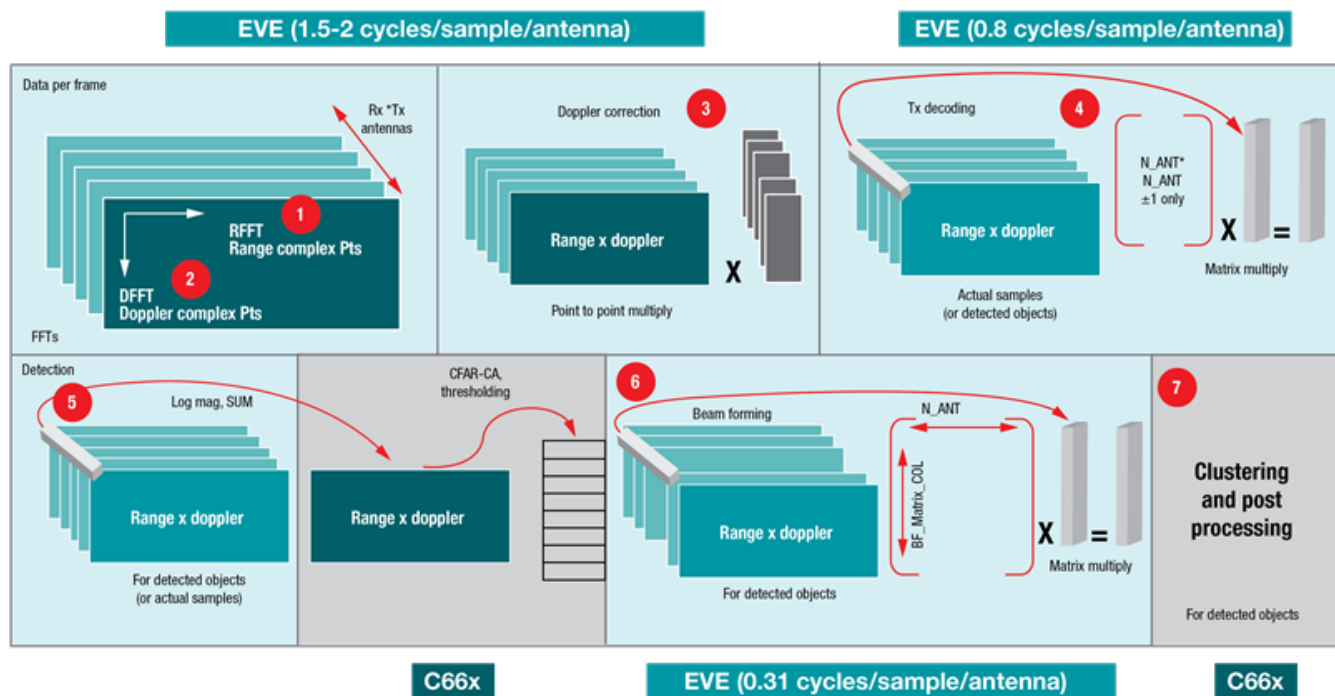
Figure 3. Radar Data Processing Flow
