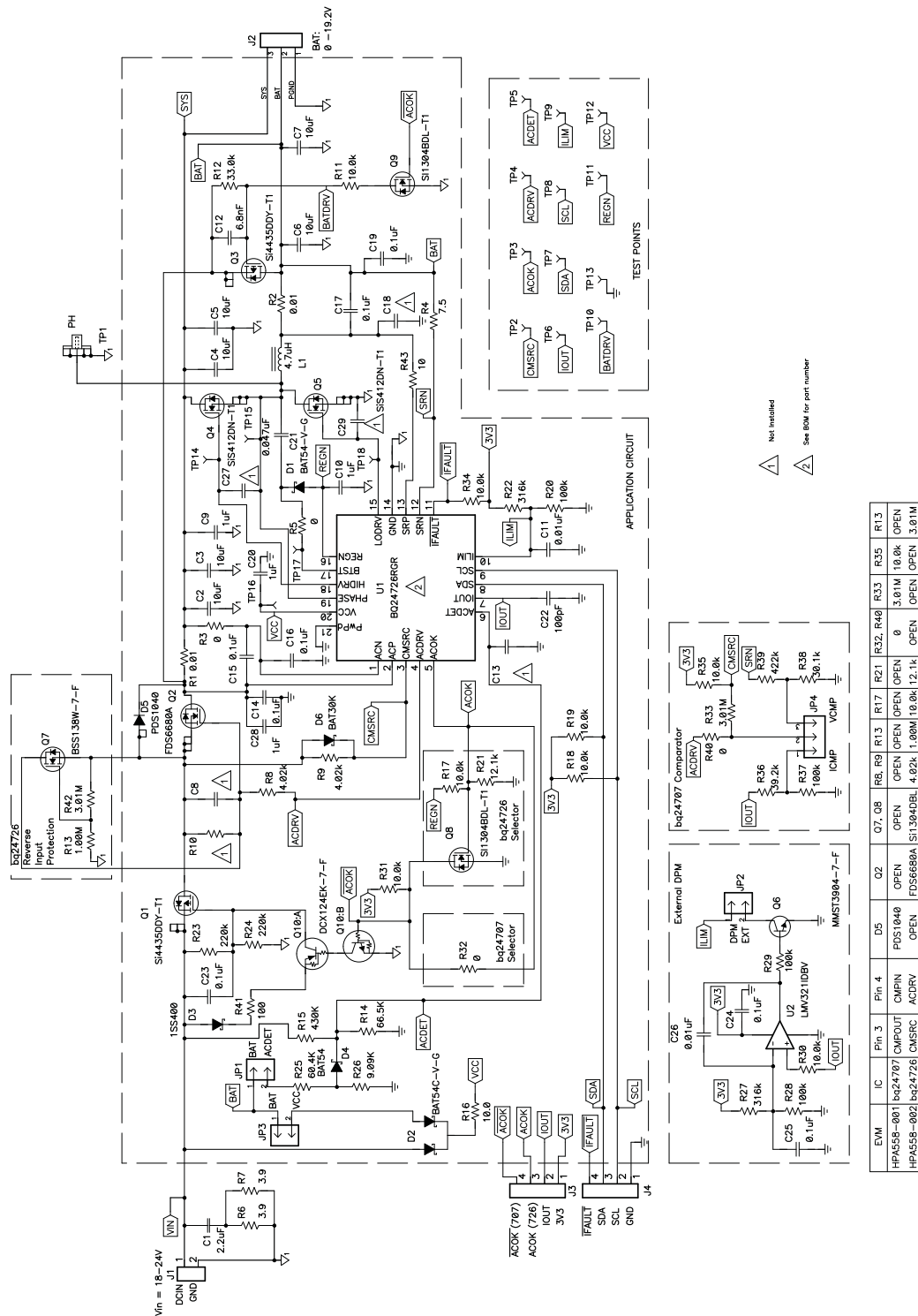
Figure 11. Schematic
