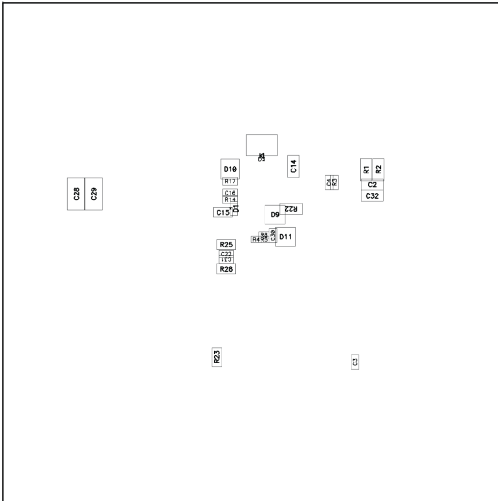
Figure 7. Bottom Assembly
