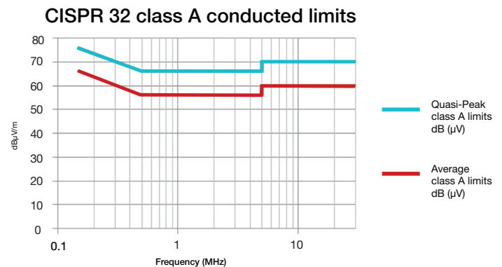
Figure 7. Graphical representation of the limits for conducted emissions from the AC mains power ports of Class A equipment defined in Table 4.
