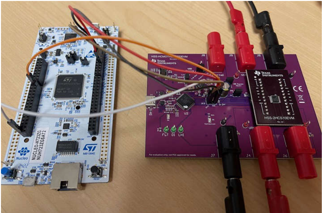
Figure 2-3. NUCLEO-H723ZG Connection
