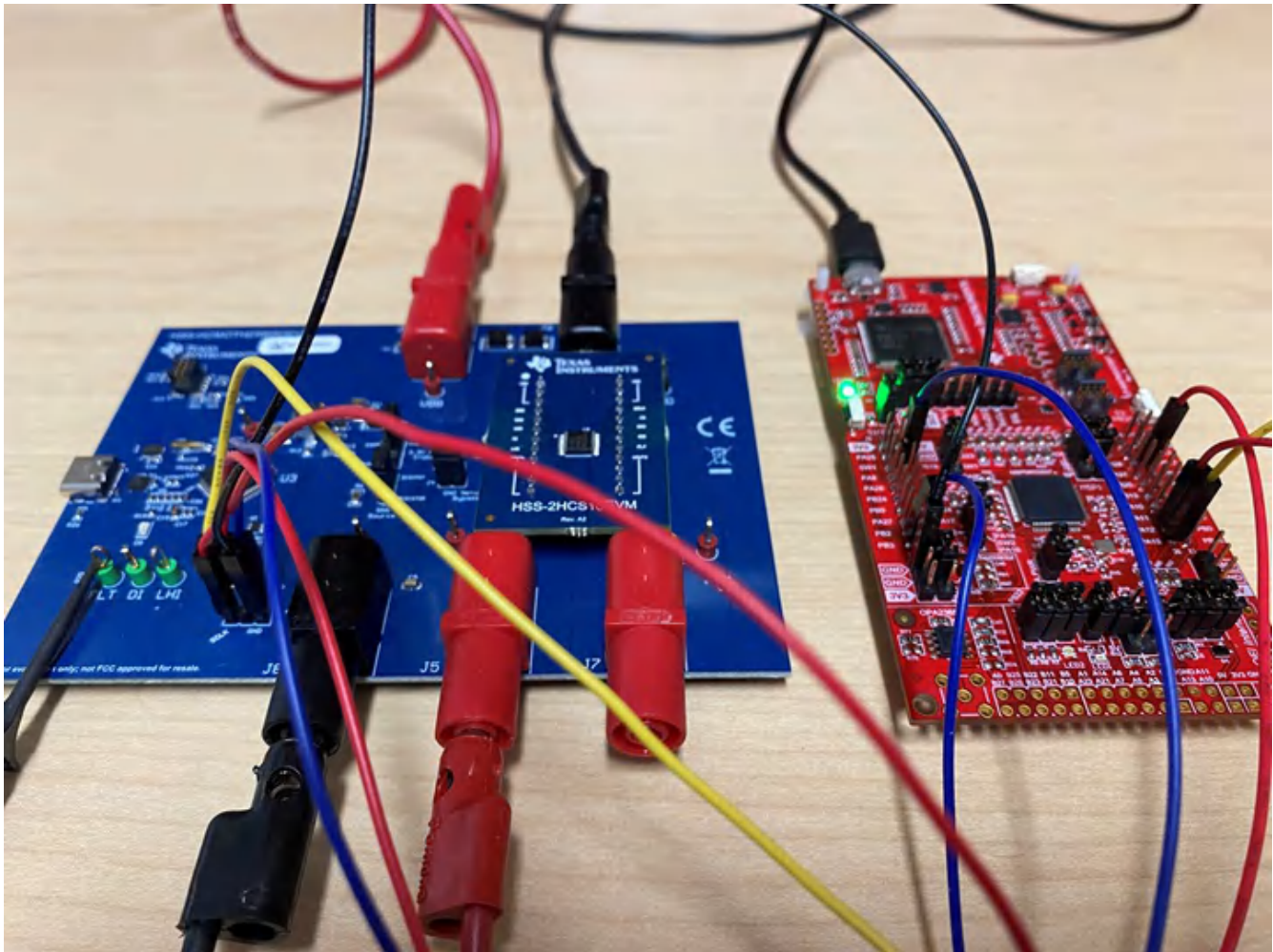
Figure 2-2. Connected MSPM0+
