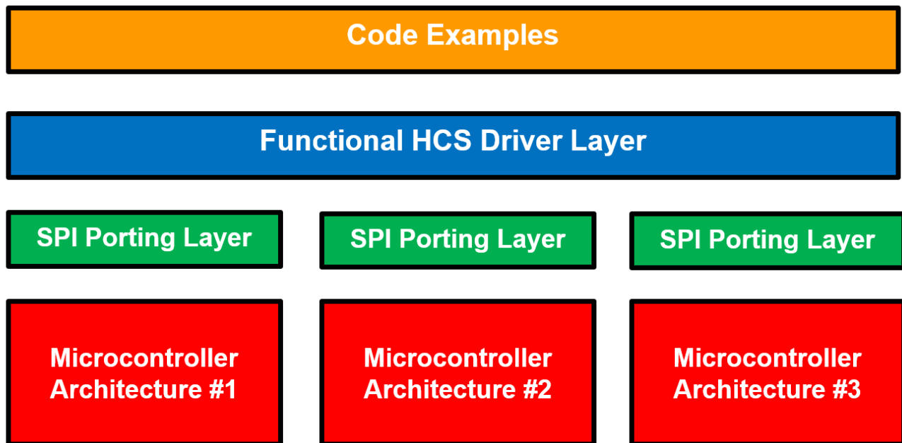
Figure 2-1. Driver Architecture
