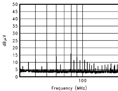
FIGURE 25b. Emissions with Addition of V_{CC} Choke
