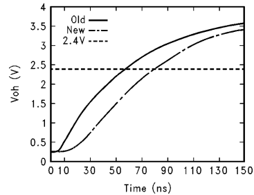
FIGURE 26b. V_{OH}
