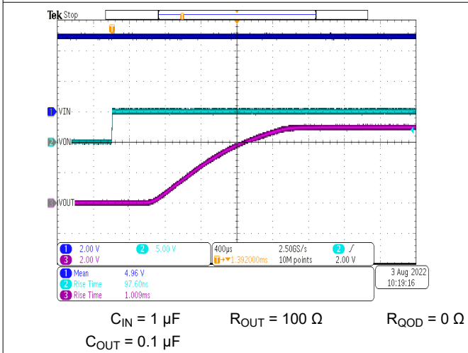
Figure 6-22. Rise Time with V_{IN} = 5 V
