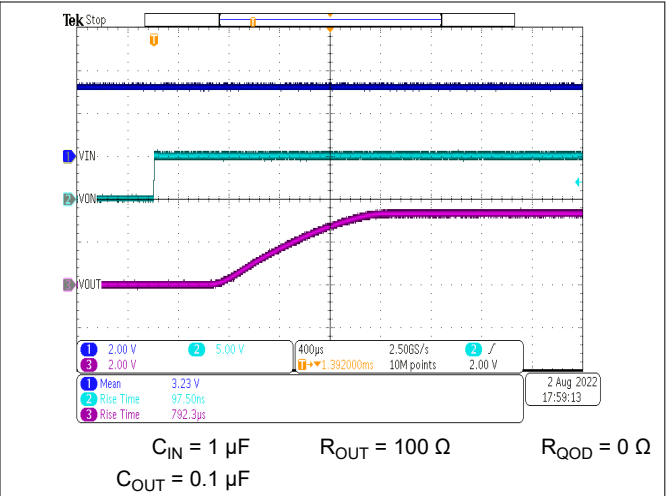
Figure 6-21. Rise Time with V_{IN} = 3.3 V
