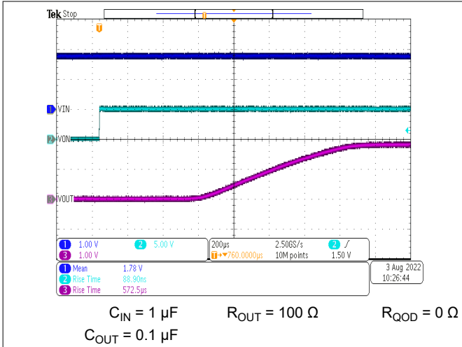
Figure 6-20. Rise Time with V_{IN} = 1.8 V
