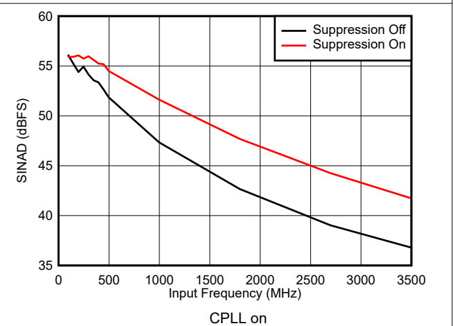
Figure 7-36. SINAD vs Input Frequency and Suppression
