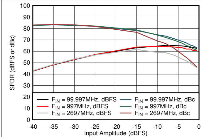
Figure 7-33. SFDR vs Input Amplitude
