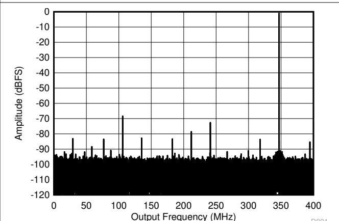
Figure 7-6. Single Tone FFT at 347 MHz and -1dBFS
