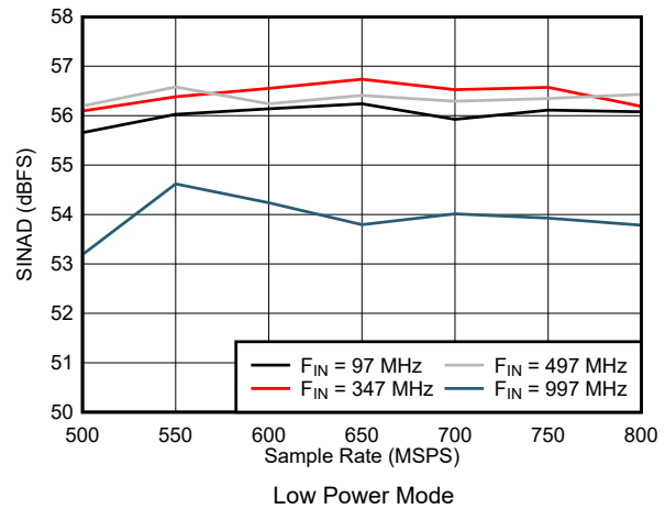
Figure 7-56. SINAD vs Sample Rate in Low Power Mode
