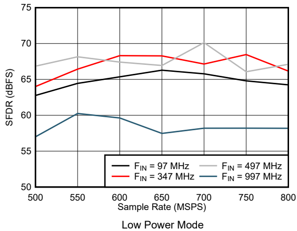
Figure 7-55. SFDR vs Sample Rate in Low Power Mode
