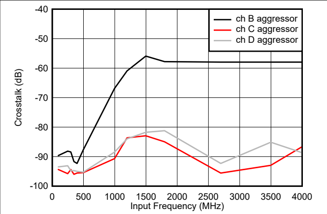
Figure 7-4. Crosstalk vs Input Frequency, Channel A victim
