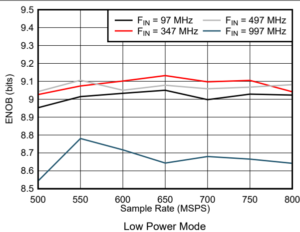
Figure 7-57. ENOB vs Sample Rate in Low Power Mode
