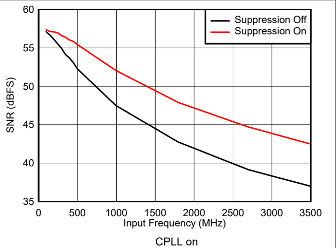
Figure 7-34. SNR vs Input Frequency and Suppression
