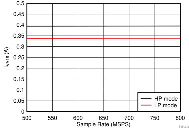
Figure 7-92. Dual Channel, I_{VA19} vs F_S Independent of JMODE
