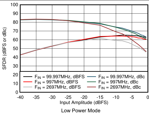
Figure 7-59. SFDR vs Input Amplitude in Low Power Mode
