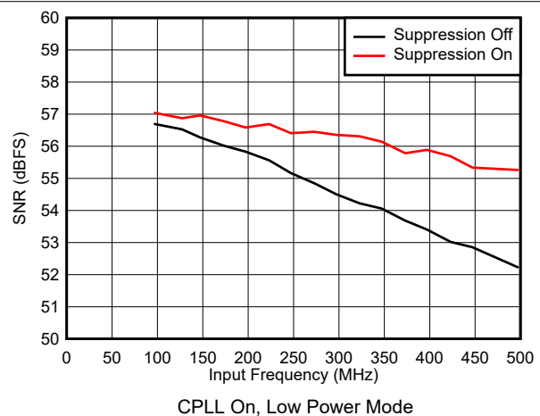
Figure 7-60. SNR vs Input Frequency
