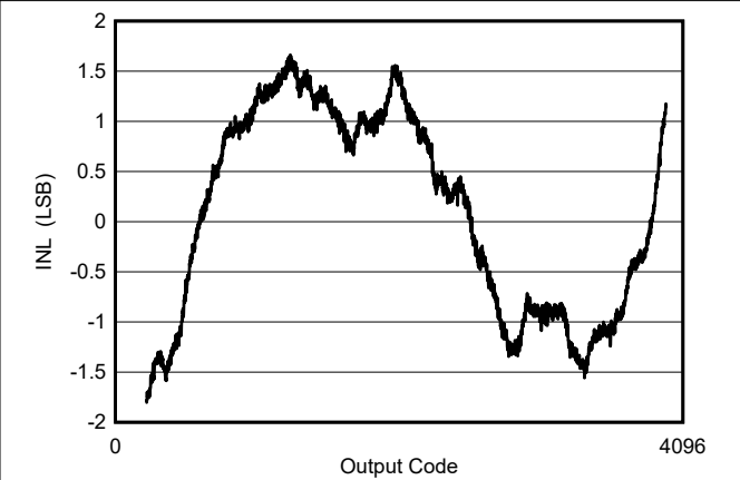
Figure 7-2. INL vs Code
