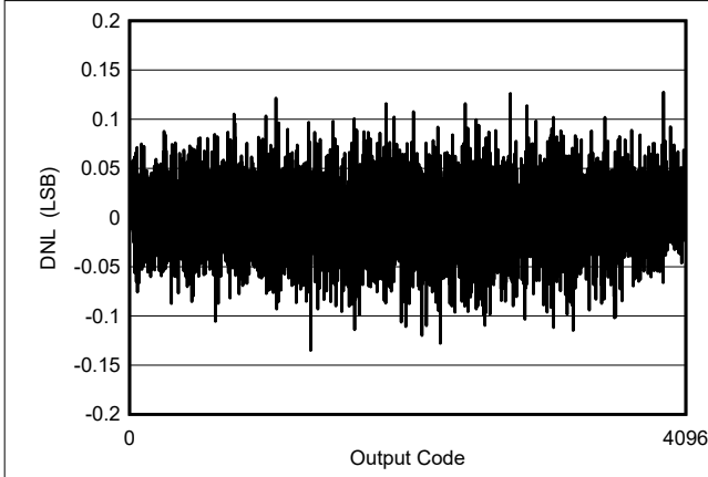
Figure 7-1. DNL vs Code
