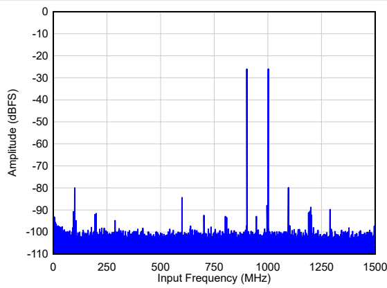
Figure 6-80. Two Tone FFT at F_{IN} = 900/1000 MHz
