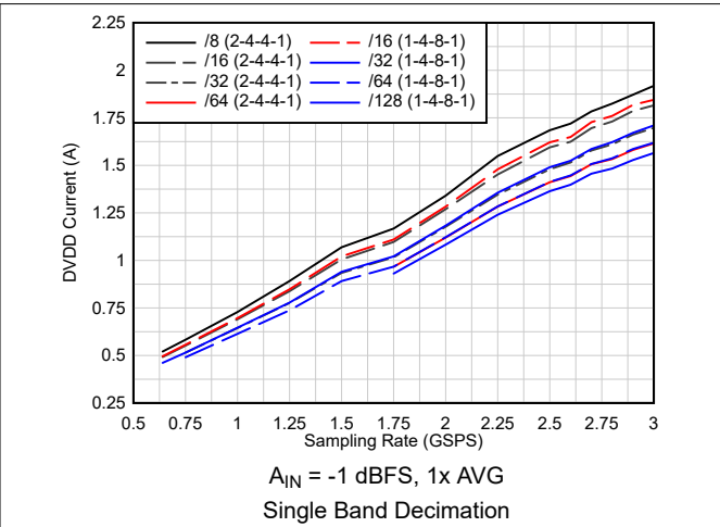
Figure 6-105. Current vs Sampling Rate vs Complex Decimation
