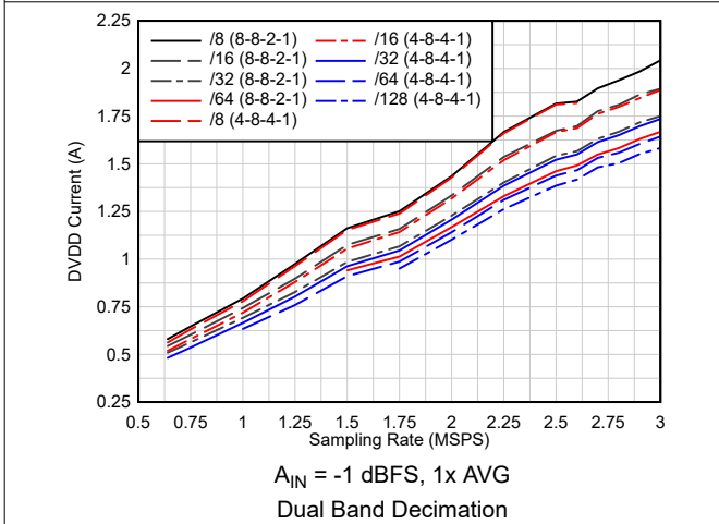
Figure 6-106. Current vs Sampling Rate vs Complex Decimation
