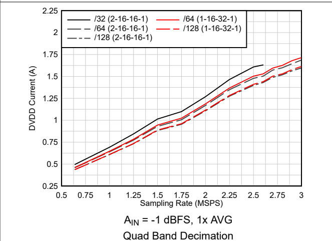
Figure 6-109. Current vs Sampling Rate vs Complex Decimation
