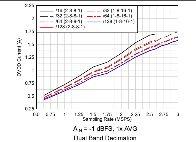
Figure 6-107. Current vs Sampling Rate vs Complex Decimation
