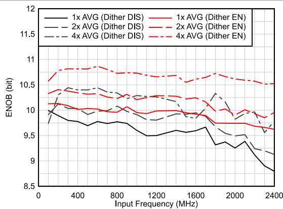
Figure 6-27. AC Performance vs F_{IN}
