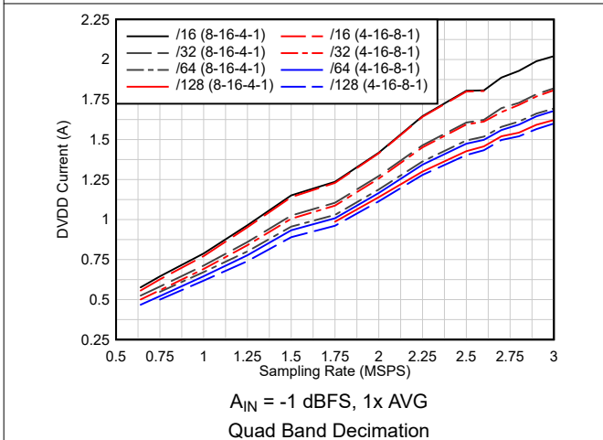
Figure 6-108. Current vs Sampling Rate vs Complex Decimation
