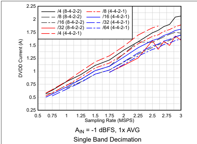
Figure 6-104. Current vs Sampling Rate vs Complex Decimation
