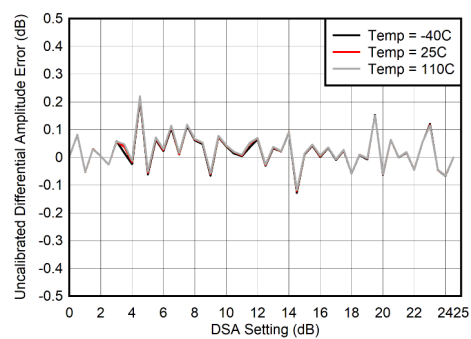
Differential Amplitude Error = P_{\text{IN}}(\text{DSA Setting} - 1) - P_{\text{IN}}(\text{DSA Setting}) + 1
