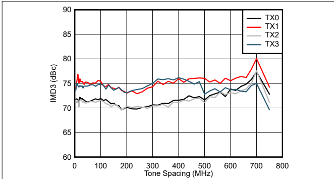
Figure 7-577. IMD3 vs Tone Spacing and Channel at 7.1 GHz
