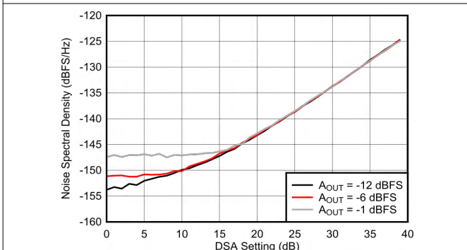
Figure 7-581. NSD vs DSA Setting and Amplitude at 7.1 GHz 50 MHz offset from tone
