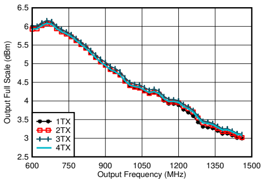
Figure 7-305. TX Full Scale vs RF Frequency and Channel at 5898.24 MSPS, Interleave Mode
