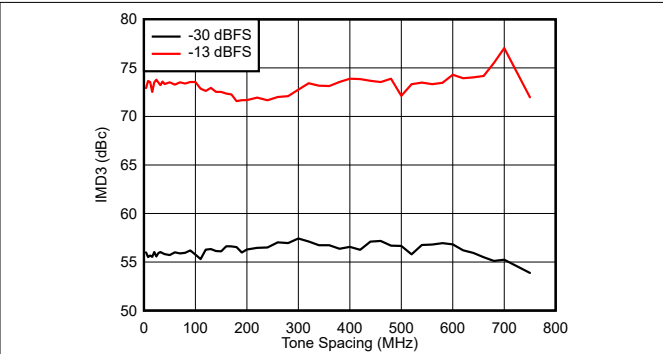
Figure 7-578. IMD3 vs Tone Spacing and Digital Amplitude at 7.1 GHz
