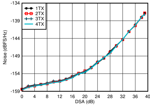
f_{DAC} = 5898.24 MSPS, interleave mode, matching at 0.8 GHz, P_{OUT} = -13 dBFS
