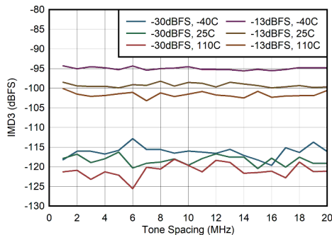
Figure 7-47. IMD3 vs Tone Spacing at 400 MHz
