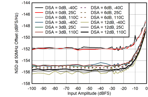
Figure 7-43. NSD vs Input Amplitude at 400 MHz
