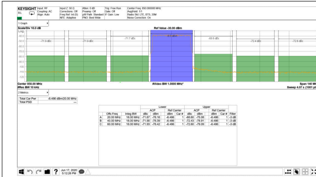
Figure 7-339. TX 20-MHz LTE Output Spectrum at 0.85 GHz
