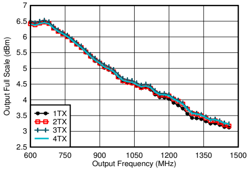
Figure 7-303. TX Full Scale vs RF Frequency and Channel at 5898.24 MSPS, Straight Mode
