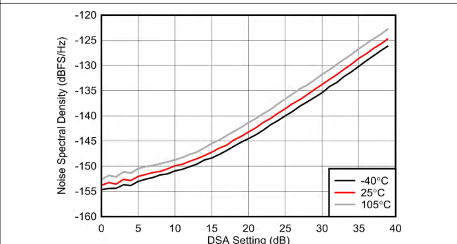
Figure 7-582. NSD vs DSA Setting and Temperature at 7.1 GHz Tone at -12 dBFS, 50 MHz offset from tone
