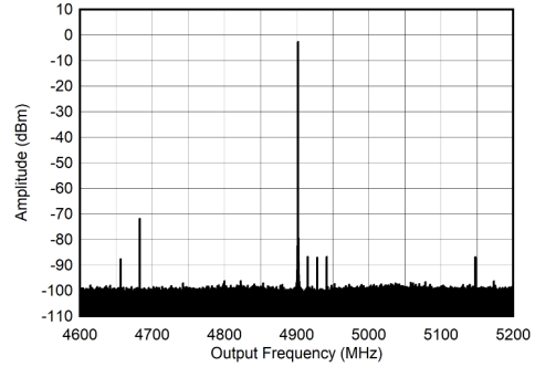
Figure 7-547. TX Single Tone (-1 dBFS) Output Spectrum at 4.9 GHz ( \pm 300 MHz)
