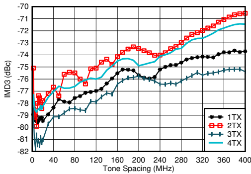
f_{DAC} = 5898.24 MSPS, straight mode, f_{CENTER} = 0.85 GHz, matching at 0.8 GHz, -13 dBFS each tone
