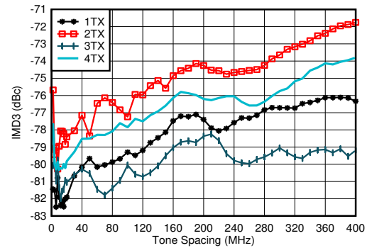
f_{DAC} = 8847.36 MSPS, straight mode, f_{CENTER} = 0.85 GHz, matching at 0.8 GHz, -13 dBFS each tone
