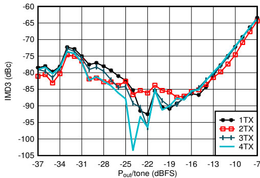
f_{\text{DAC}} = 11796.48 MSPS, interleave mode, f_{\text{CENTER}} = 0.85 GHz, f_{\text{SPACING}} = 20 MHz, matching at 0.8 GHz
