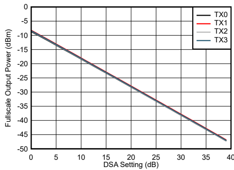
Figure 7-555. TX Full Scale vs DSA Setting and Channel at 7.1 GHz
