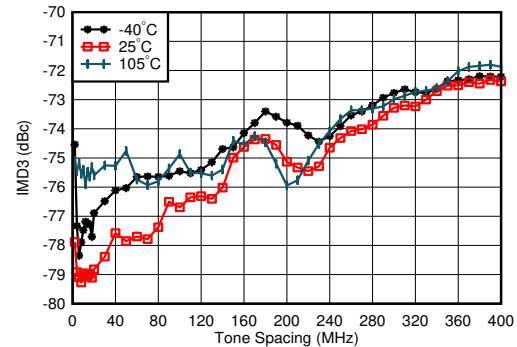
f_{DAC} = 5898.24 MSPS, straight mode, f_{CENTER} = 0.85 GHz, matching at 0.8 GHz, -13 dBFS each tone, worst channel
