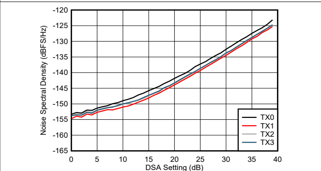
Figure 7-580. NSD vs DSA Setting and Channel at 7.1 GHz Tone at -12 dBFS, 50 MHz offset from tone
