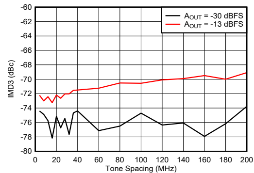
f_{\text{DAC}} = 9000 MSPS, non-interleave mode, external clock mode Figure 6-437. IMD3 vs Tone Spacing and Amplitude at 2.6 GHz
