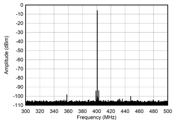
Figure 6-274. Single Tone Spectrum at 400 MHz and -12 dBFS ( \pm 100\text{MHz} )
