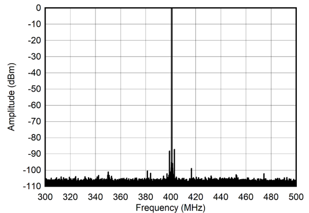
Figure 6-272. Single Tone Spectrum at 400 MHz and -6 dBFS ( \pm 100\text{MHz} )
