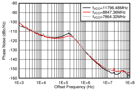
Figure 6-592. Phase Noise vs Offset Frequency and f_{\text{VCO}} at f_{\text{OUT}} = 2610 \text{ MHz}
