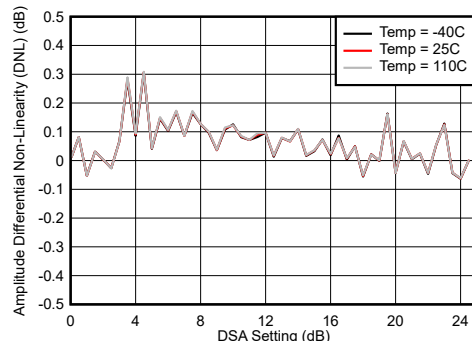
Figure 6-2. RX Uncalibrated Differential Amplitude Error vs DSA Setting at 30 MHz
