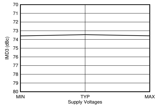
f_{\text{DAC}} = 11796.48 MSPS, interleave mode, 2.6 GHz matching. 40-MHz offset from tone. Output Power = -13 dBFS. All supplies simultaneously at MIN, TYP, or MAX voltages. Figure 6-435. TX IMD3 vs Supply Voltage at 2.6 GHz
