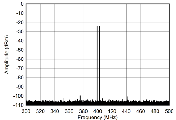
Figure 6-284. Dual Tone Spectrum at 400 MHz and -30 dBFS ( \pm 100 MHz)
