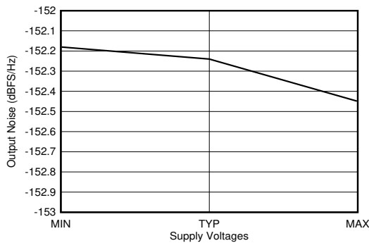
f_{\text{DAC}} = 11796.48 MSPS, interleave mode, 2.6 GHz matching. 40-MHz offset from tone. Output Power = -1 dBFS. All supplies simultaneously at MIN, TYP, or MAX voltages. Figure 6-434. TX Output Noise vs Supply Voltage at 2.6 GHz
