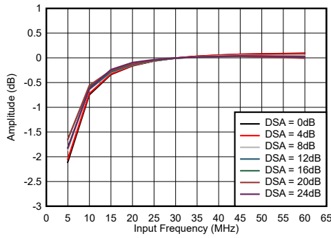
Figure 6-1. RX In-Band Gain Flatness, f_{\text{IN}} = 30 MHz
