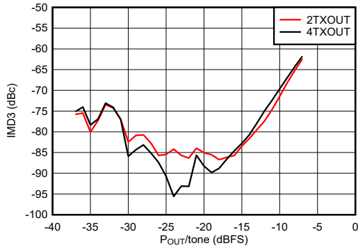
f_{DAC} = 5898.24 MSPS, straight mode, f_{CENTER} = 0.85 GHz, f_{SPACING} = 20 MHz, matching at 0.8 GHz
