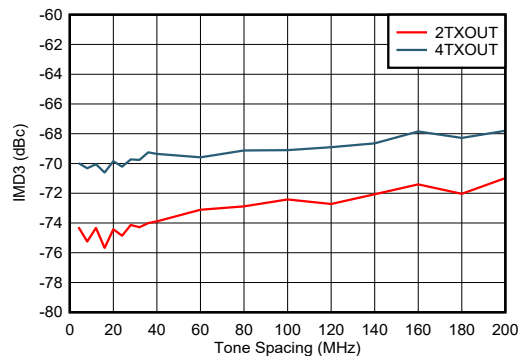
f_{\text{DAC}} = 9000 MSPS, non-interleave mode, external clock mode Figure 6-436. IMD3 vs Tone Spacing and Channel at 2.6 GHz
