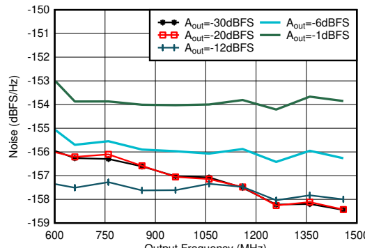
Matching at 0.8 GHz, Single tone, f_{DAC} = 11.79648 GSPPS, interleave mode, 40-MHz offset, DSA = 0dB
