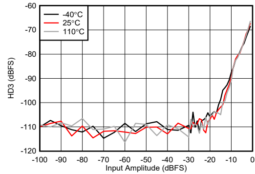
Figure 6-162. RX HD3 vs Input Level at 3.76GHz
