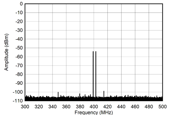
Figure 6-286. Dual Tone Spectrum at 400 MHz and -60 dBFS ( \pm 100 MHz)
