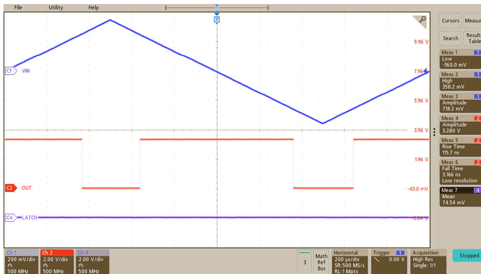
Figure 8-3. Output Response of the AMC22C12-Q1 to a Triangular Input Waveform
