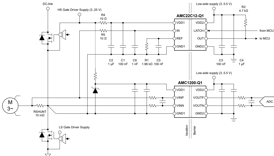
Figure 8-1. Using the AMC22C12-Q1 for Overcurrent Detection
