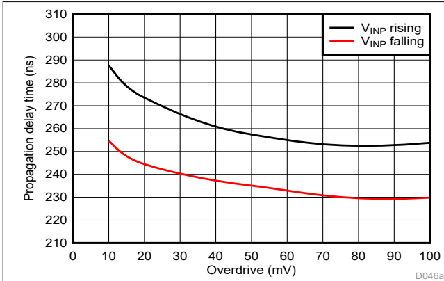
Figure 6-35. Cmp0 Propagation Delay vs Overdrive
