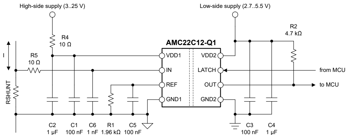
Figure 8-6. Decoupling of the AMC22C12-Q1
