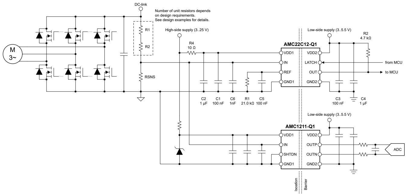
Figure 8-2. Using the AMC22C12-Q1 for Overvoltage Detection
