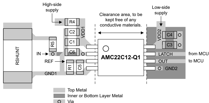
Figure 8-7. Recommended Layout of the AMC22C12-Q1
