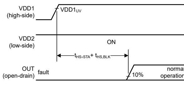
Figure 7-6. VDD2 is On; VDD1 Turns On (Long Delay)
