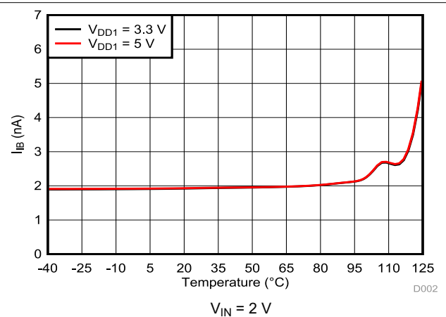
Figure 6-40. Input Bias Current vs Temperature
