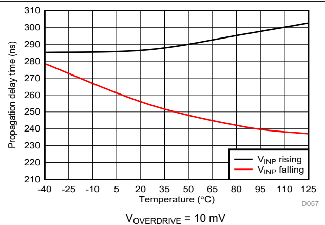
Figure 6-36. Cmp0 Propagation Delay vs Temperature
