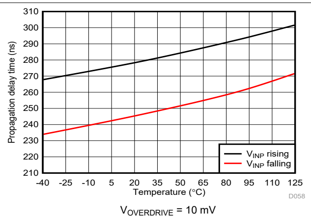
Figure 6-38. Cmp1 Propagation Delay vs Temperature
