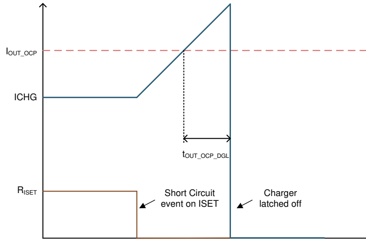
Figure 7-4. Overcurrent Protection
