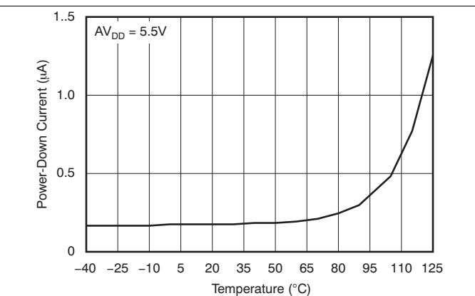
Figure 31. Power-Down Current vs Temperature
