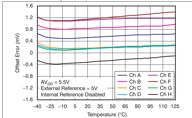
Figure 26. Offset Error vs Temperature
