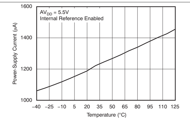
Figure 29. Power-Supply Current vs Temperature
