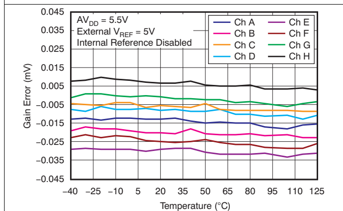
Figure 30. Gain Error vs Temperature
