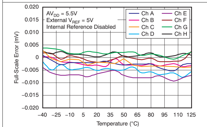
Figure 28. Full-Scale Error vs Temperature
