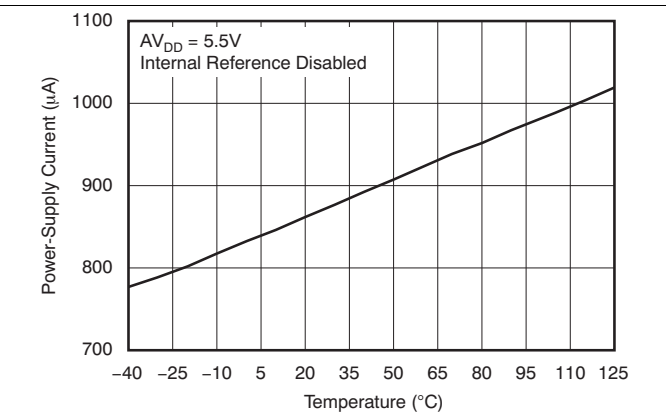
Figure 27. Power-Supply Current vs Temperature
