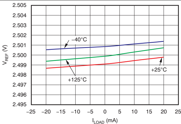
Figure 10. Internal Reference Voltage vs Load Current (Grades C and D)
