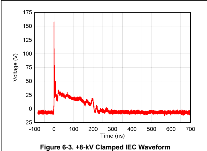
Figure 6-3. +8-kV Clamped IEC Waveform
