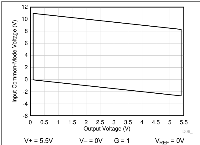
Figure 6-71. Input Common-Mode Voltage vs Output Voltage (Rail-to-Rail CMRR Region)
