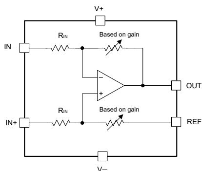
INA500 Simplified Internal Schematic
