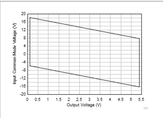
Figure 6-72. Input Common-Mode Voltage vs Output Voltage (High CMRR Region)
