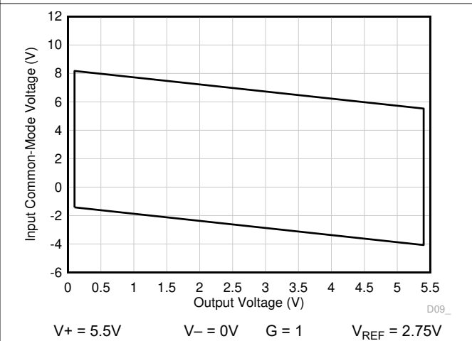
Figure 6-74. Input Common-Mode Voltage vs Output Voltage (High CMRR Region)
