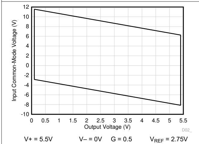
Figure 6-73. Input Common-Mode Voltage vs Output Voltage (High CMRR Region)
