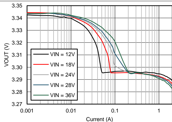
Figure 49. Output Voltage Regulation
