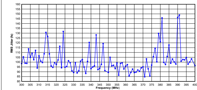
Figure 6-19. RMS Jitter vs Frequency (300MHz to 400MHz) for LVPECL, HCSSL; TYPICAL 3.3V, 25°C
