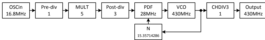
Figure 8-23. Frequency Plan in PLL Duplex Mode
