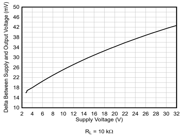
Figure 5-36. Output Swing vs Supply Voltage, Positive Swing
