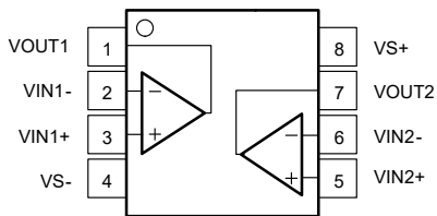
Figure 5-2. OPA2863A D Preview Package, 8-Pin SOIC and DGK Preview Package, 8-Pin VSSOP (Top View)
