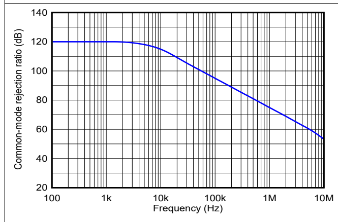
Figure 6-44. Common-Mode Rejection Ratio vs Frequency
