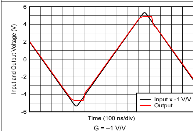
Figure 6-11. Output Overdrive Recovery
