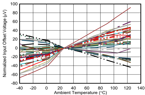
Normalized to 25^\circ\text{C} values, 35 units, DSN package
