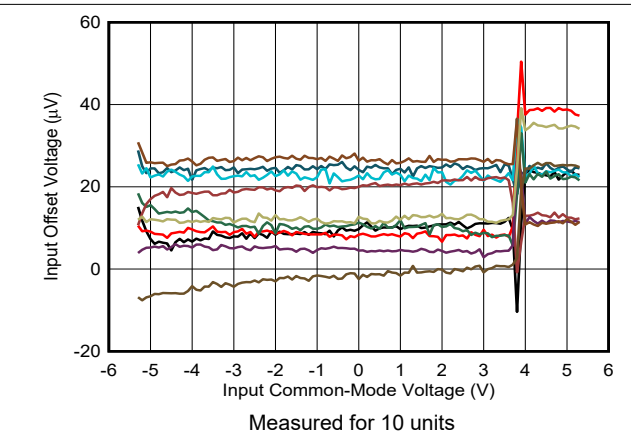
Figure 6-12. Input Offset Voltage vs Input Common-Mode Voltage
