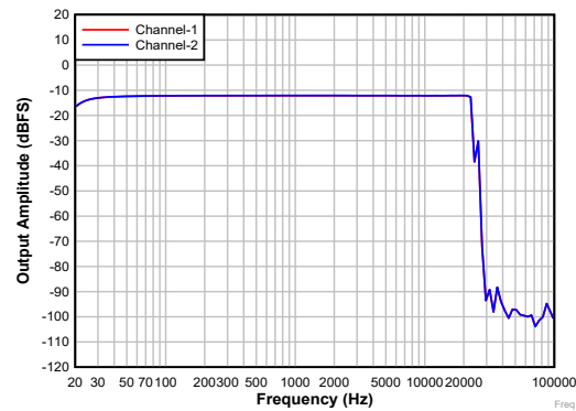
Figure 7-6. Differential Input: Frequency Response With a -12\text{-dBr} Input
