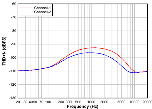
Figure 7-5. Differential Input: THD+N vs Input Frequency With a -1\text{-dBr} Input
